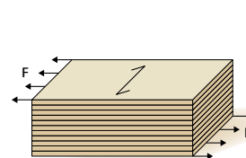
M f_{v,90,flat} and G_{90,flat} Flat-wise, perp. to grain♦♦
